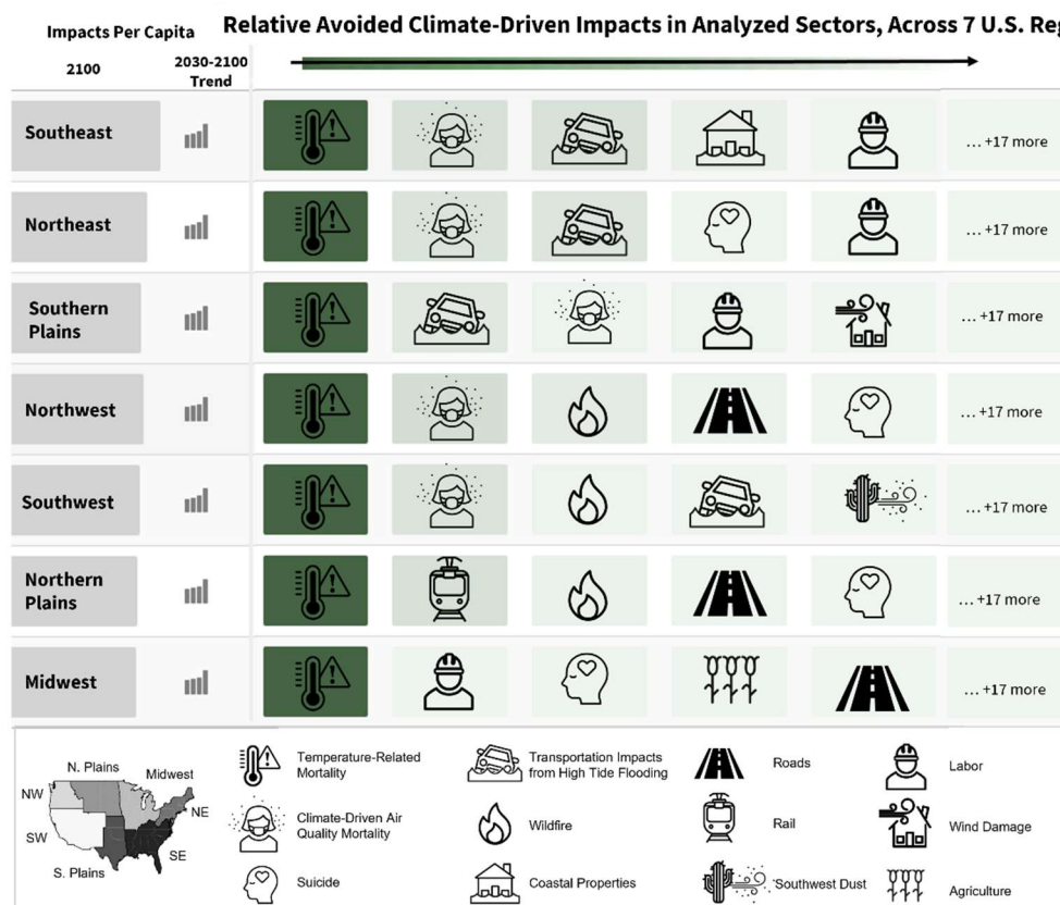
Figure B-2 Relative avoided per capita climate driven impacts by sector and US region in 2100. 90
