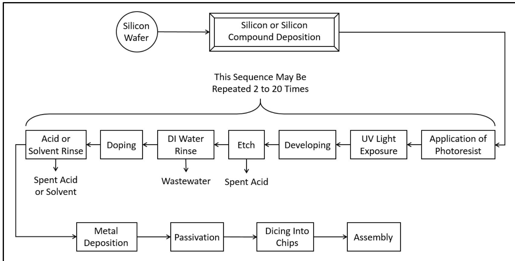
Figure 1. 1983 Silicon Integrated Circuit Production
