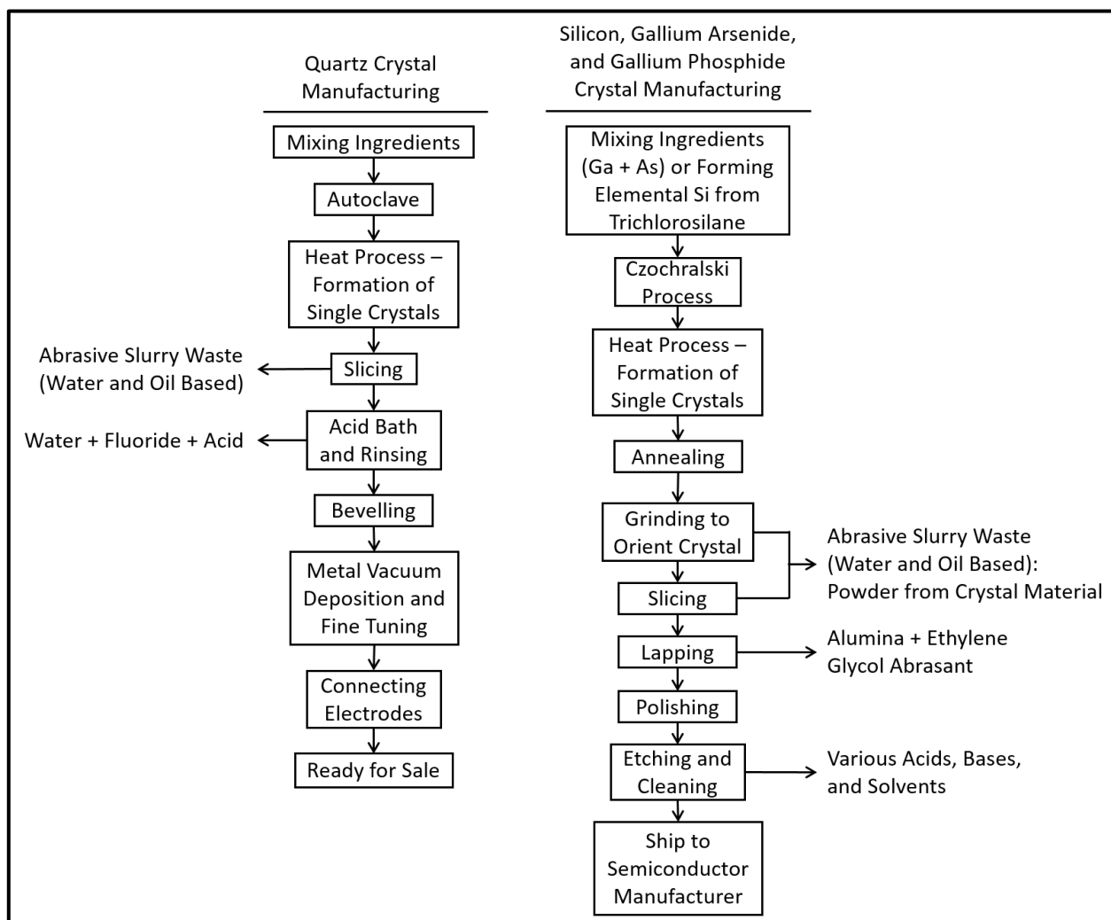
Figure 2. Basic Manufacturing Processes for Electronic Crystals in 1983
