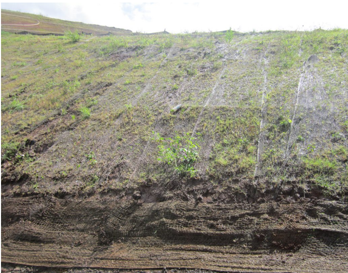
Geotextile matting can be used on slopes to help establish vegetation by protecting the soil surface and seedlings from erosion while still allowing vegetation to grow through the mat.
