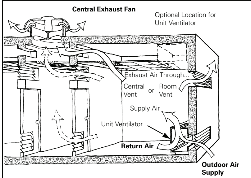
Air Supply through a Unit Ventilator
